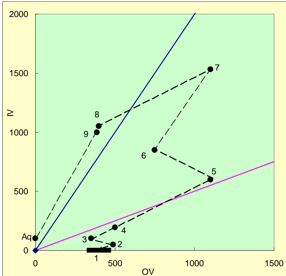
Figure 28, Organic Conceptual Diagram of Formulation
