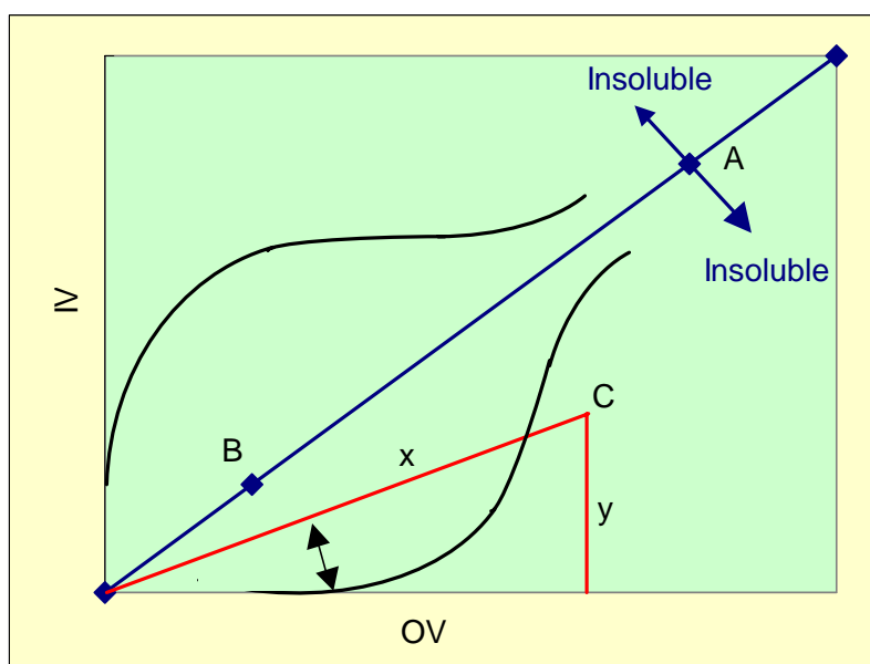
Figure 7, Properties of Organic Conceptual Diagram
