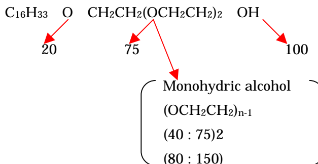
Figure 4, Organic Conceptual Diagram of Typical Non-Ion Surfactant
