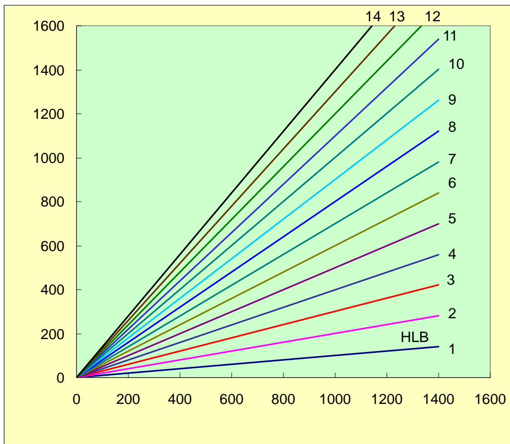
Figure 10, HLB of Oda type and Conceptual Diagram
