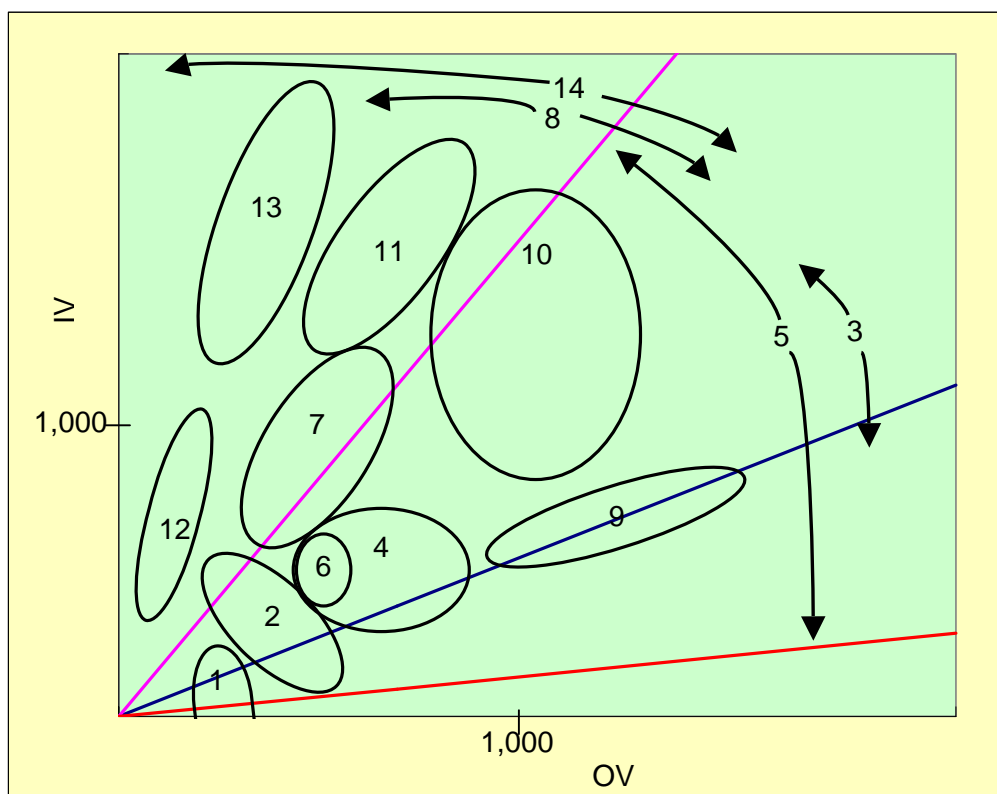
Figure 8, Conceptual Diagram of similar compounds
